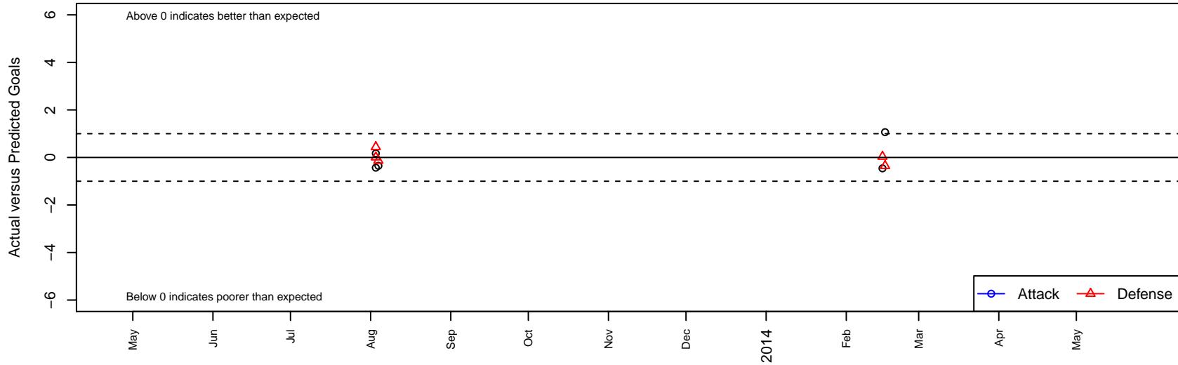
Rush Soccer SPI Select G99 Dots are actual minus expected GF (blue circles) and GA (red triangles). Blue line is smoothed change in attack strength. Red is smoothed change in defense strength.
